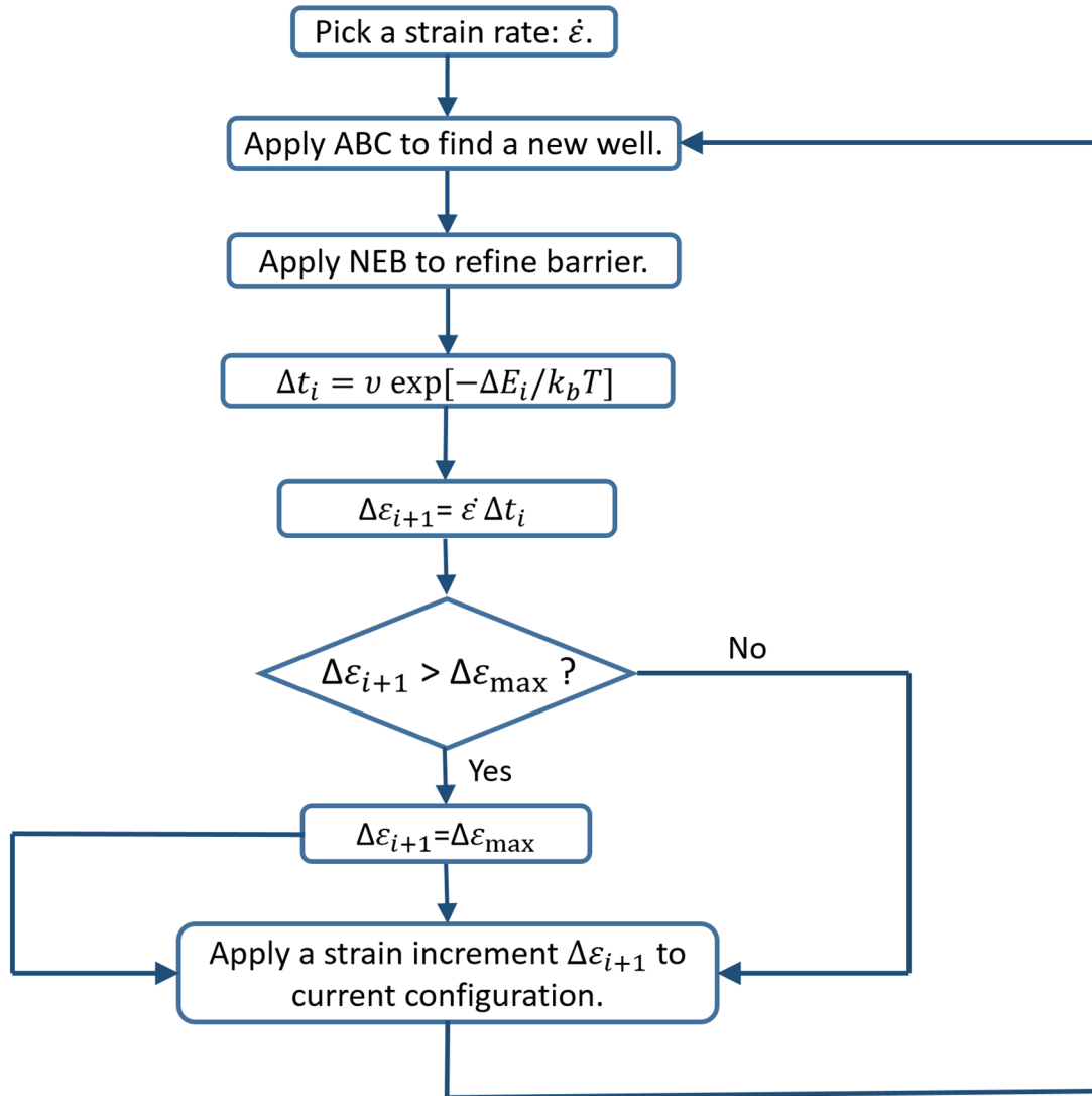
Figure 7. Algorithmic flowchart for method 5 [62].
