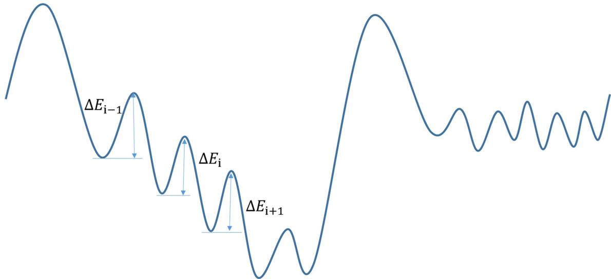
Figure 1. Schematic of a one-dimensional potential energy surface.
