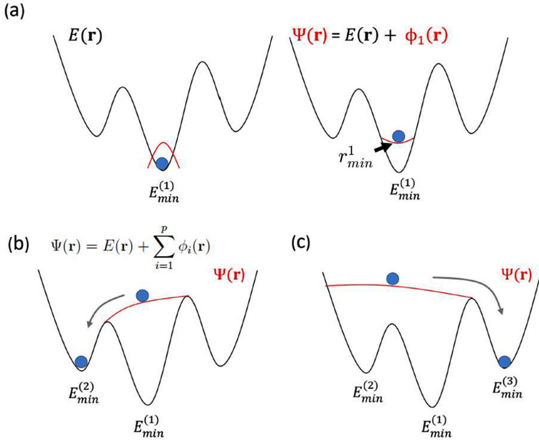
Figure 2. Illustration of basin filling with penalty functions in the ABC method. (a) Penalty function \phi_1 added to PES, with the center of the penalty functions at \mathbf{r}_{min}^i ; ((b) and (c)) continue adding additional penalty functions to push the system to neighboring energy wells. Adapted from [39] with permission. Copyright 2014 Elsevier.
