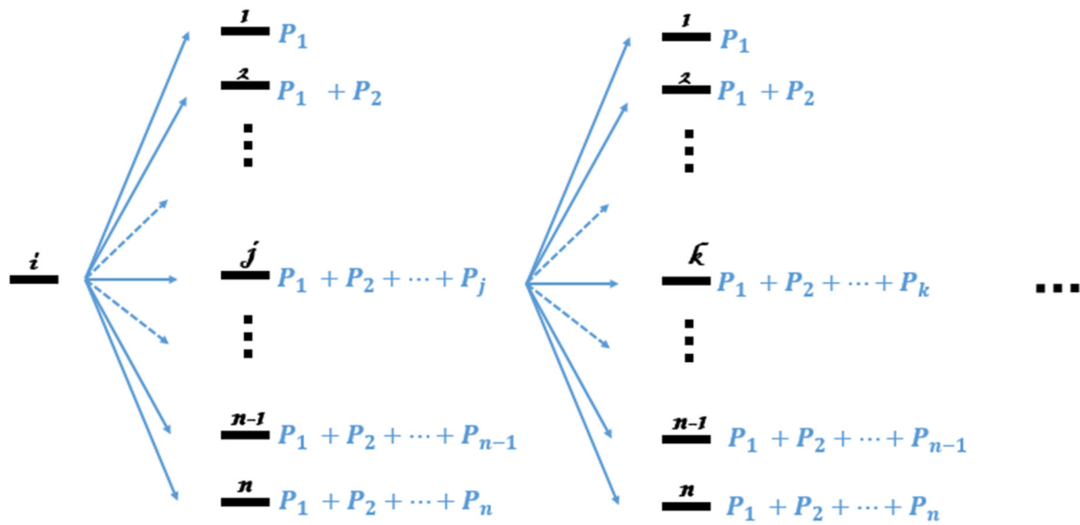
Figure 4. KMC algorithm: Starting from the state i , a random number ( r ) in the range of (0,1] is compared with the partial summation of possibilities and it turns out P_1 + P_2 + \dots + P_{j-1} < r < P_1 + P_2 + \dots + P_j . Thus, the system will jump to state j . State j becomes the current state and the same action will be taken with state j . Reprinted from [43] with permission. Copyright 2015 Elsevier.
