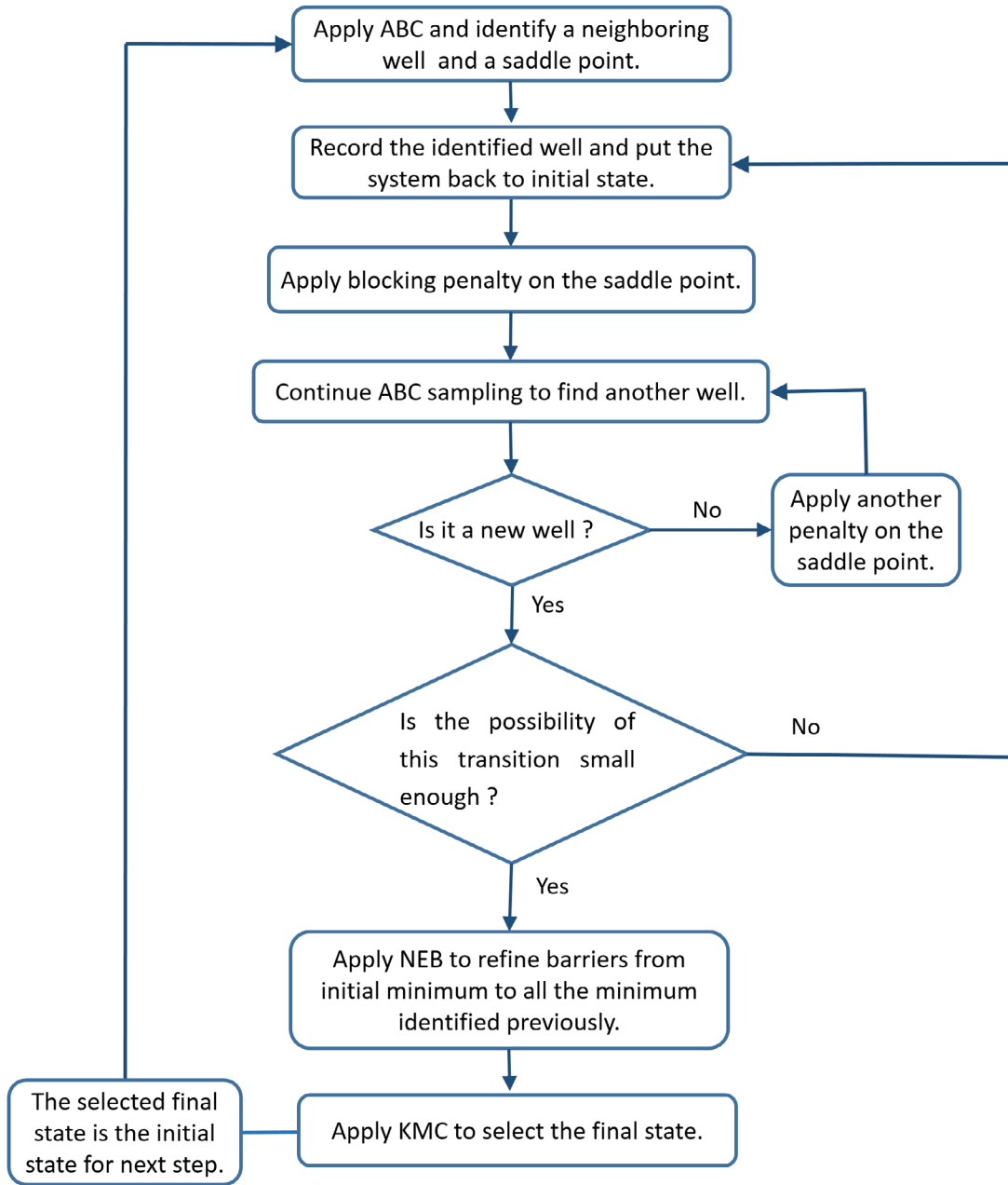
Figure 5. Algorithmic flowchart of method 3 (ABC-E) [19].
