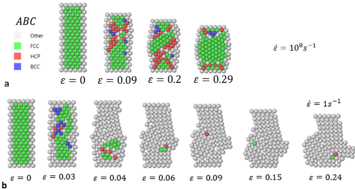
Figure 13. Ni compression under different strain rates. (a) Fast, MD-like strain rate. (b) Slow, experimentally-relevant strain rate. Reproduced with permission from [69]. Copyright 2016 American Chemical Society.
